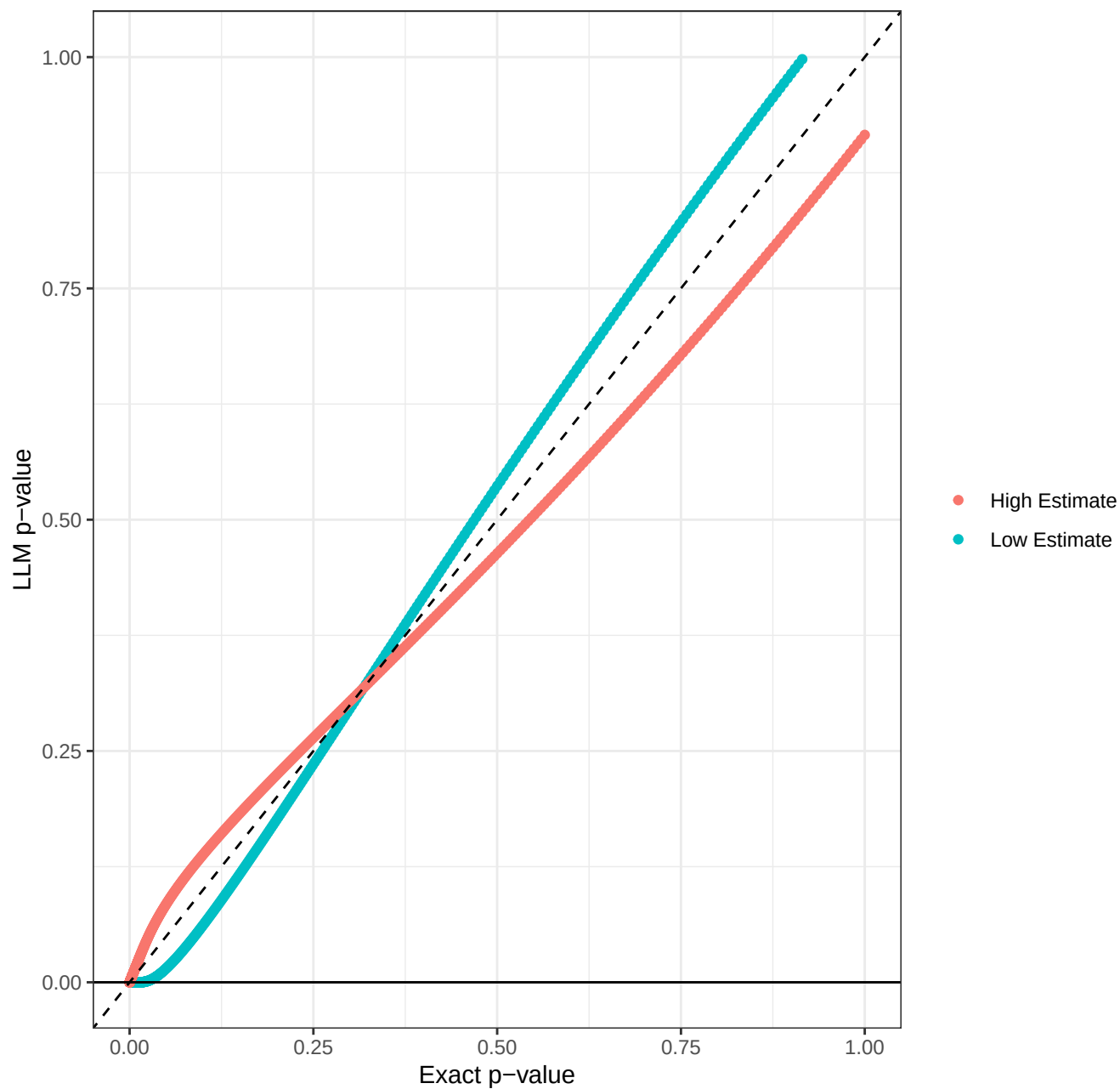
Exact vs. LLM Approach
